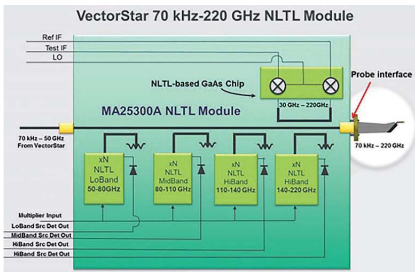
3. Thanks to a direct dc-path transmission line from the VNA, the ME7838G offers optimum raw directivity. The waveguide bands are coupled to that transmission line.
