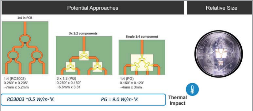
4. A variety of approaches can be taken to implement a 1:4 feed.
