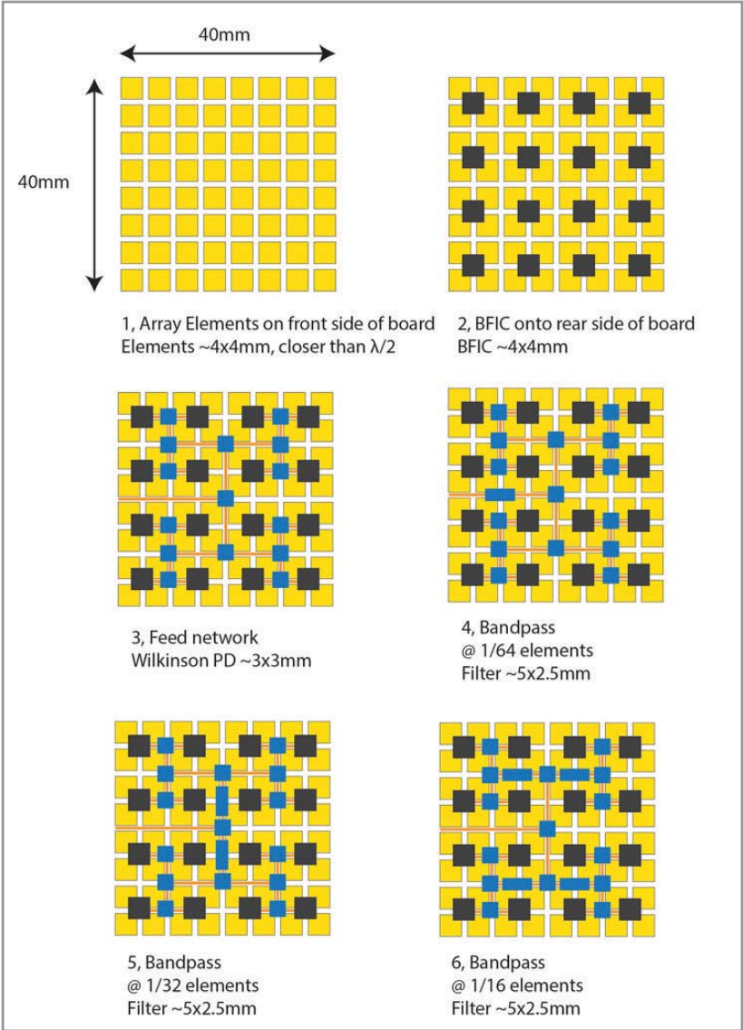
2. RF component dimensions are constrained by the size of the array.
